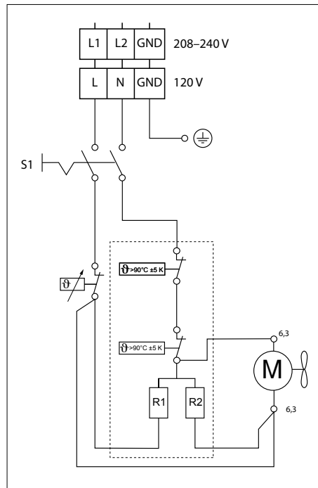
Wiring diagram CK 150-1 Plus, CK 200-2 Plus
