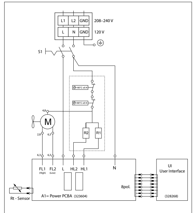
Wiring diagram CK 150-1 Premium, CK 200-2 Premium
